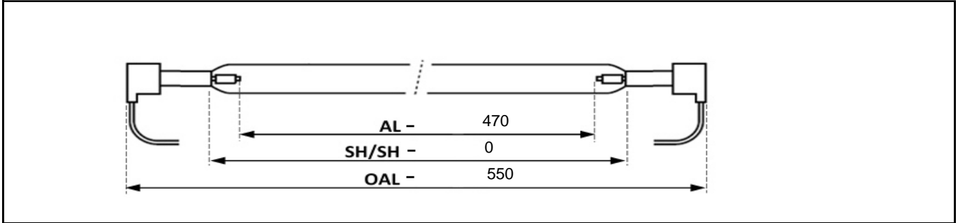
Socket Diagram:
